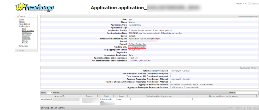
图 3-6 application
