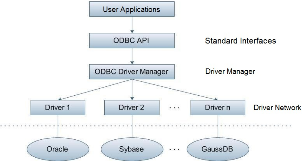
Figure 12-2 ODBC system structure
