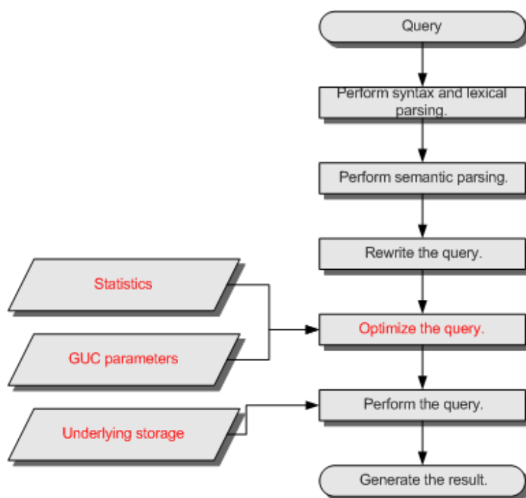
Figure 14-2 Execution process of query-related SQL statements by the SQL engine
