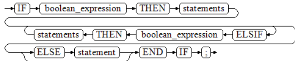
Figure 10-18 IF_THEN_ELSEIF_ELSE::=
