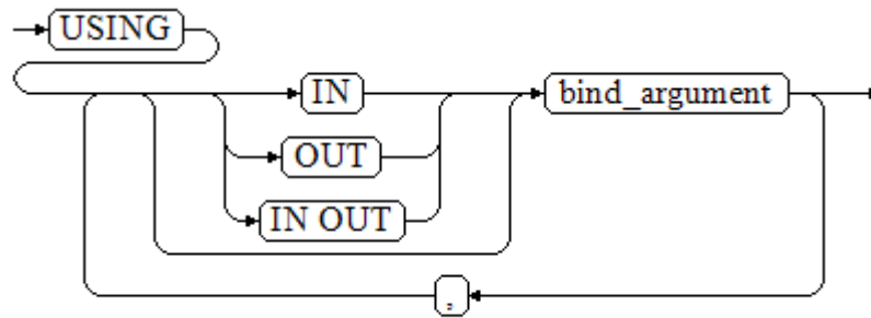
Figure 10-14 using_clause-4
