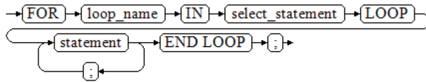
Figure 10-33 FOR_AS_loop::=
