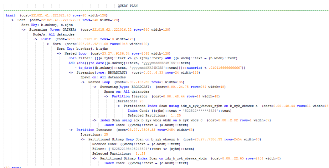
Figure 14-6 Using an unlogged table (1)
