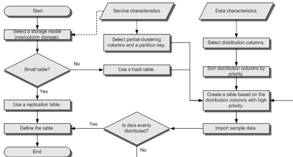
Figure 14-5 Defining a table
