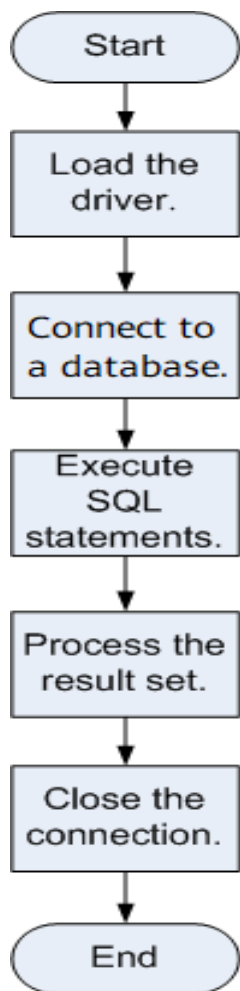
Figure 12-1 JDBC-based application development process
