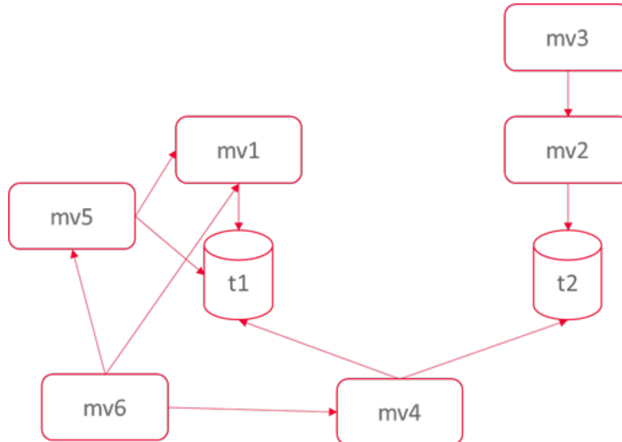
Figure 8-1 Dependency between nested materialized views
