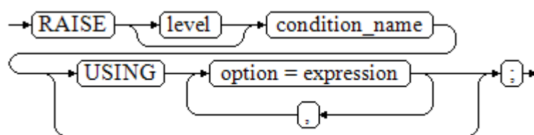
Figure 10-35 raise_condition::=
