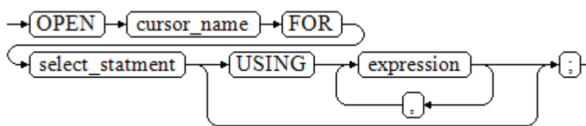
Figure 10-30 open_dynamic_cursor::=
