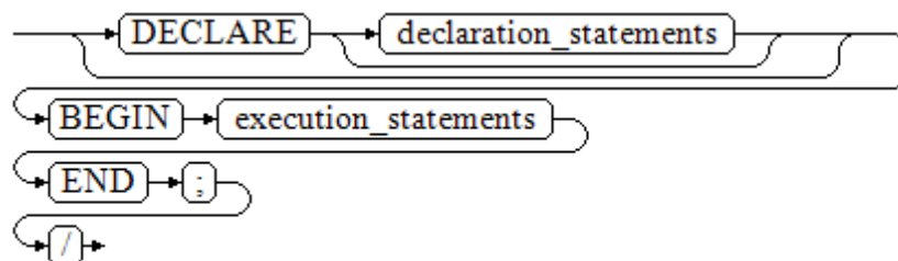
Figure 10-2 anonymous_block::=
