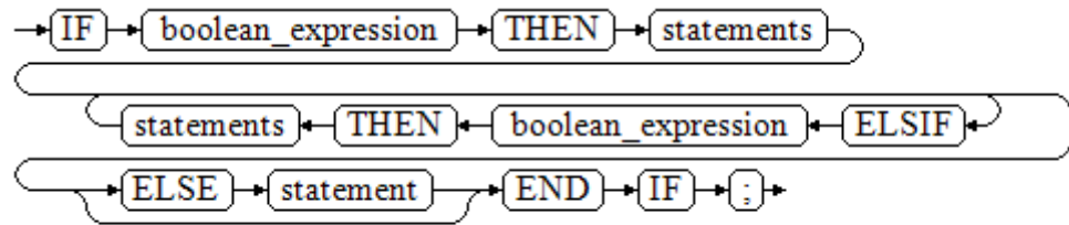
Figure 10-18 IF_THEN_ELSEIF_ELSE::=
