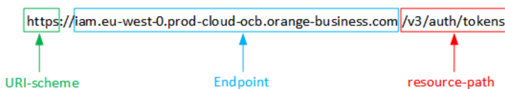
Figure 3-1 Example URI
