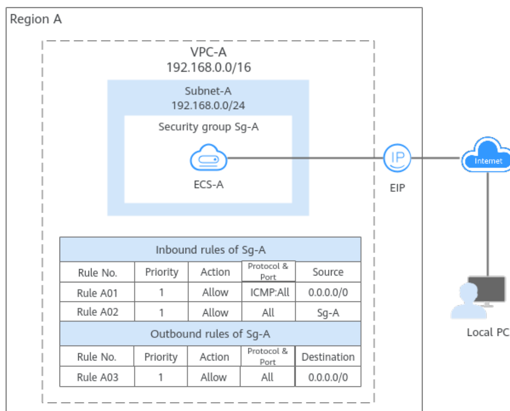
Figure 8-6 A security group architecture
