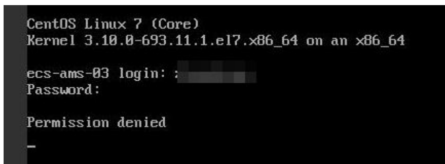
图 16-103 Permission denied
